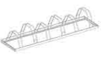
J17461 Bicycle rack, 6 bikes L x W x H: 2000 mm x 500 mm x 350 mm Hot-dip galvanized. Free standing.
