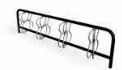
NF7620A Urban A double sided bicycle rack L x W x H: 2080 mm x 400 mm x 550 mm Underground concrete foundation.
