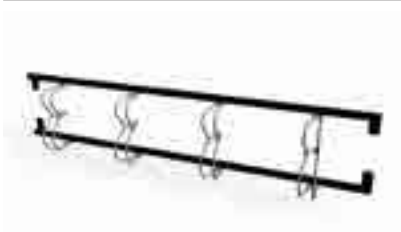
NF7600A Urban A bicycle rack L x W x H: 2050 mm x 200 mm x 570 mm Wall mounting.
