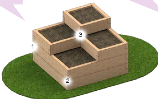
Height of tiers Tier 1: 450mm Tier 2: 300mm Tier 3: 600mm
